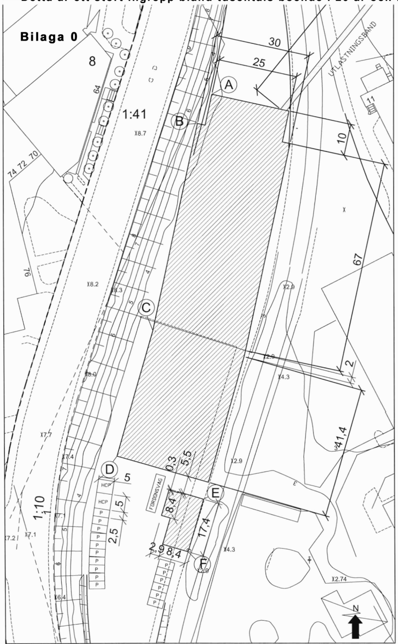
SITUATIONSPLAN
